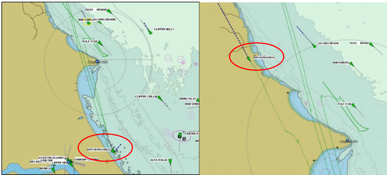
Figure 10: AIS traces as observed from the MCA station at Flamborough. Note the recorded trace of NLV Pole Star as she passed through the GPS service denial region. The trace not only extends further north and south than the true passage, it also shows the vessel crossing the land. The location of “Dutch Progress” is also marked as her position changes due to erroneous GPS input to her AIS.
