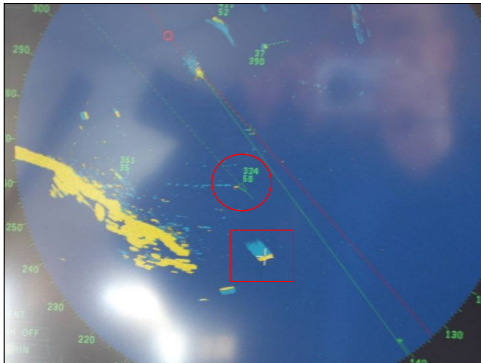
Figure 9 : Photo of NLV Pole Star 's radar with AIS overlay: Note the yellow crosshair (red square) indicates the radar return of vessel "33458" whose AIS position is reported to be some distance to the North (red circle).
