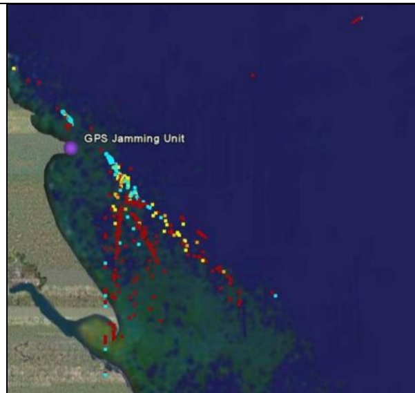
Figure 7 : Google Earth™ plot of recorded positions identified as valid, with GPS jamming unit active.
