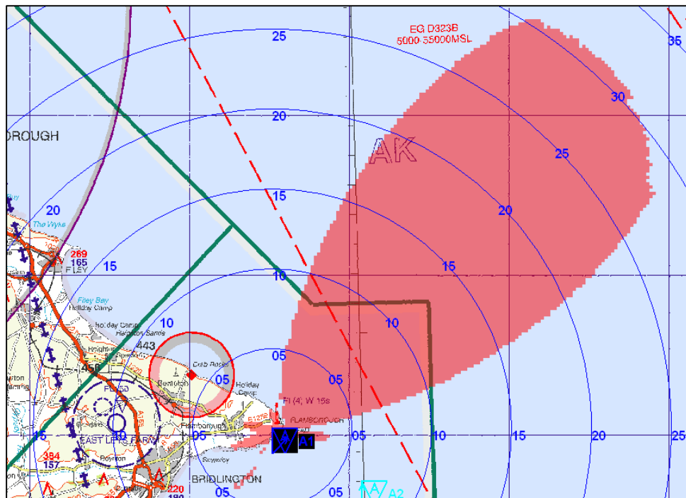
Figure 2 : Coverage area of the GPS jamming unit at 25m above ground level on maximum power of 1.58W ERP. (Image courtesy of DSTL)
