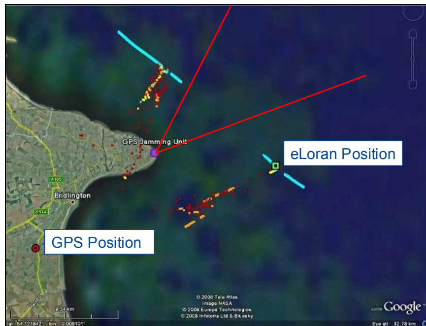
Figure 8 : Google Earth™ Plot of valid GPRMC data from one of the typical marine grade receivers with the comparison of an erroneous GPS position (red circle) against the eLoran position (green square) for the same time. The GPS position is reported as being inland 22Km West from the true eLoran position. (Red lines indicate main lobe of the jamming unit and position colours indicate reported speed: blue <15knts, yellow < 50knts, orange <100knts and red >100knts)
