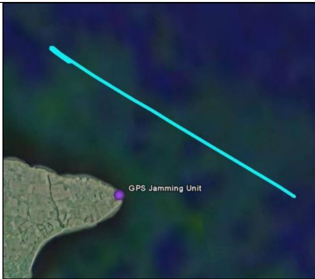
Figure 6 : Google Earth™ plot of recorded positions identified as valid, with no GPS jamming unit active.
