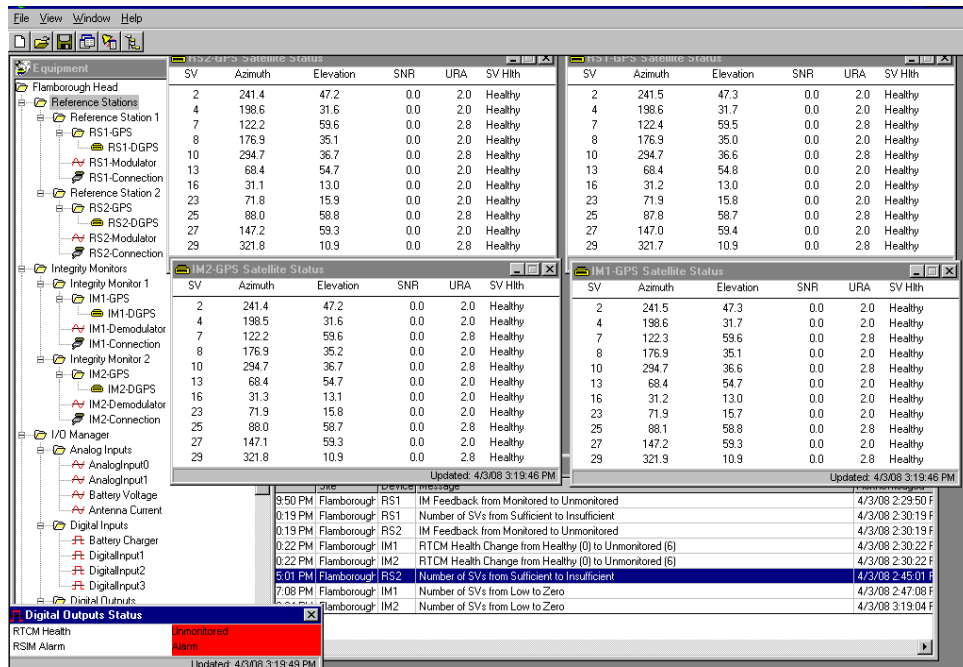
Figure 5: Screen shot of the Beacon Control Software (TM) at Flamborough Head showing that the Signal-to-Noise ratios (SNR) for all satellites on both reference stations and on both integrity monitors (4 windows to the top right of the image) are zero and that this has led to the station issuing an alarm (red area at the bottom left of the screen).
