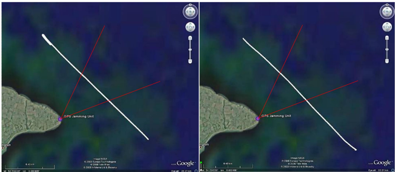
Figure 4 : Two plots of eLoran data displayed in Google Earth™. The left-hand plot is the reported positions during a control run when there was no GPS jamming. The right-hand plot shows the reported positions during a run with GPS jamming switched on. The red lines indicate the approximate boundaries of the main lobe of the GPS jamming signal. eLoran was not affected by GPS jamming.
