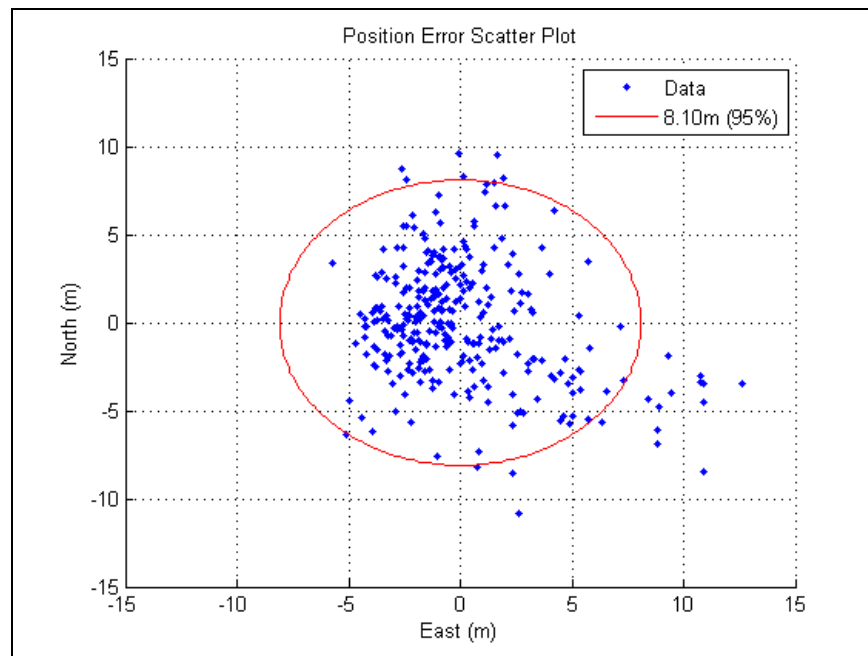
Figure 3: Scatter plot showing the performance of calibrated Loran when compared to Differential GPS. Loran was accurate to 8.1m (95%).
